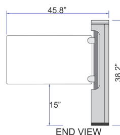
END VIEW
